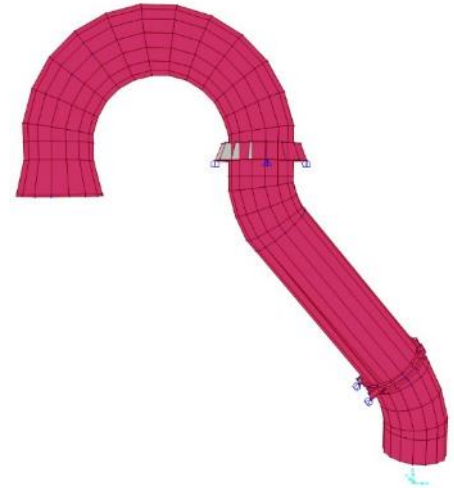
PIURA - Ducts, Raw Meal Grinding Plant
